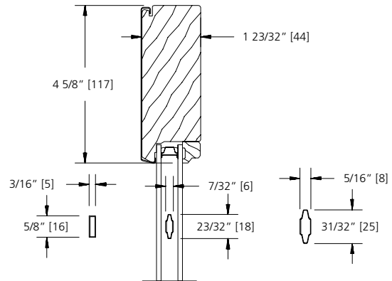
5/8" FLAT GBG
