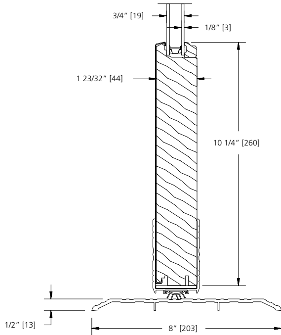
OPTIONAL 10 1/4" BOTTOM RAIL HANDICAP SILL (4 9/16" JAMB)
