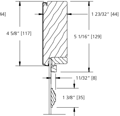
1 3/8" FULL SURROUND
