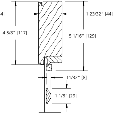
1 1/8" FULL SURROUND
