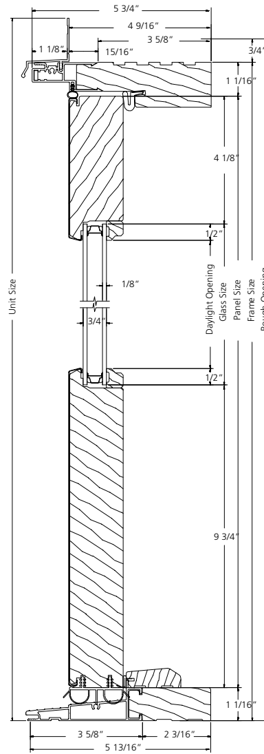
VERTICAL SECTION
