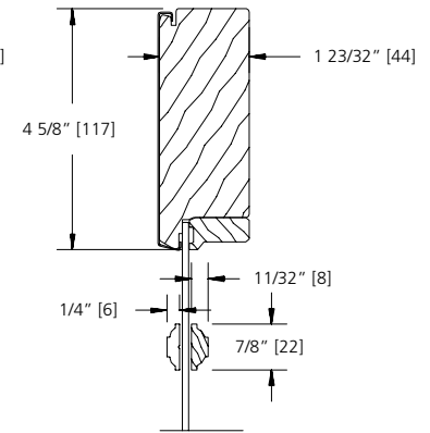
7/8" SDL BAR (BEAD STOP)
