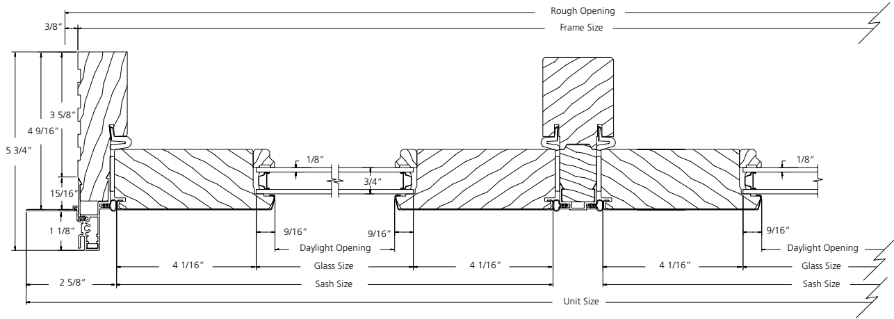
HORIZONTAL SECTION
