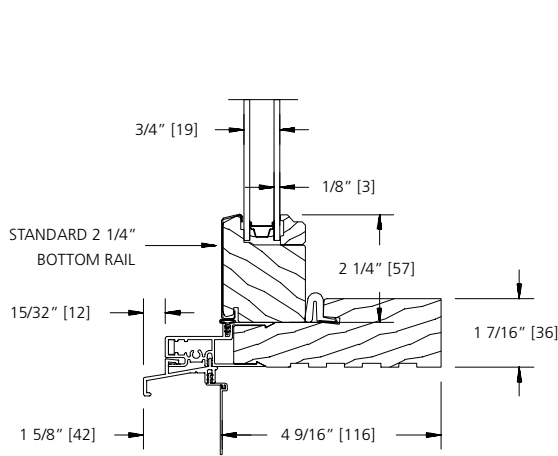
TRANSOM SILL NOSE (4 9/16" JAMB)
