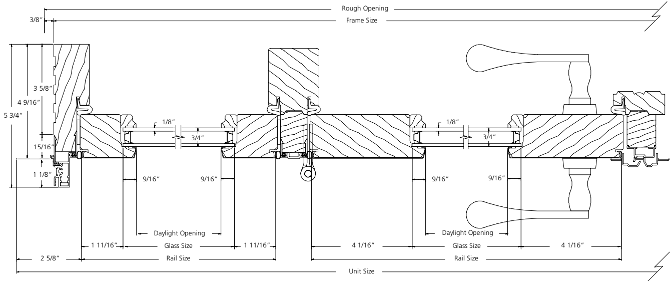
HORIZONTAL SECTION
