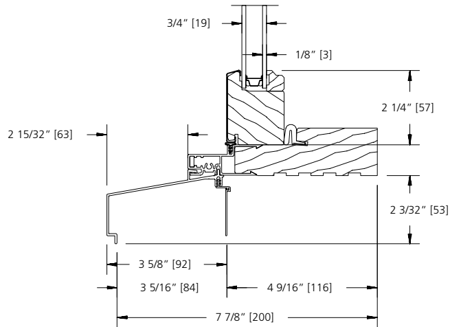
TRANSOM EXTENDED SILL NOSE (4 9/16" JAMB)
