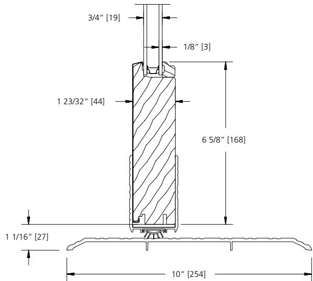
STANDARD 6 5/8" BOTTOM RAIL HANDICAP SILL (6 9/16" JAMB)
