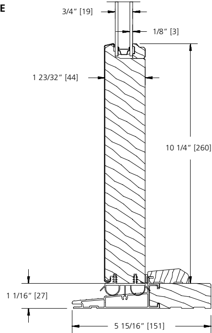
OPTIONAL 10 1/4" BOTTOM RAIL STANDARD SILL (4 9/16" & 6 9/16" JAMB)
