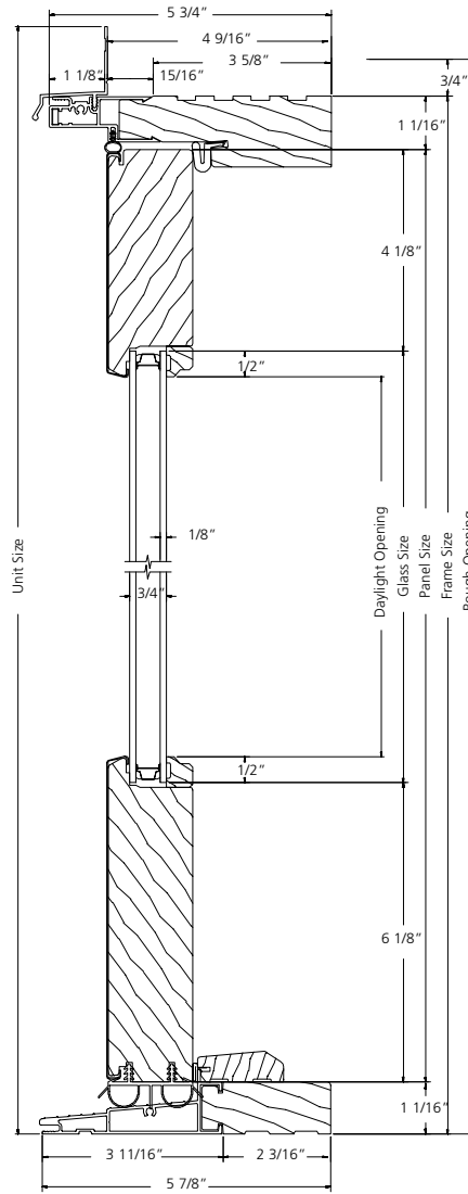
VERTICAL SECTION
