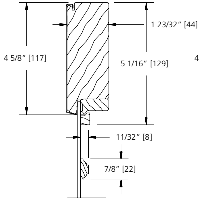
7/8" FULL SURROUND
