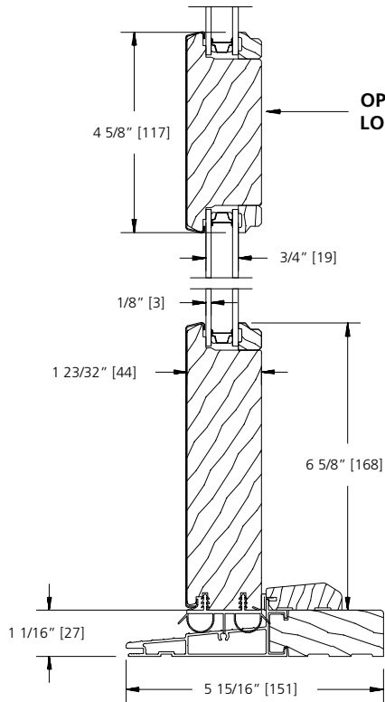
STANDARD 6 5/8" BOTTOM RAIL STANDARD SILL (4 9/16" & 6 9/16" JAMB)
