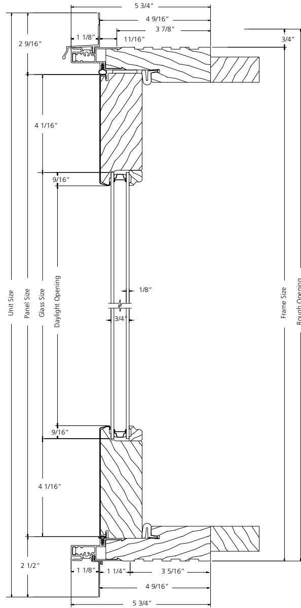
VERTICAL SECTION
