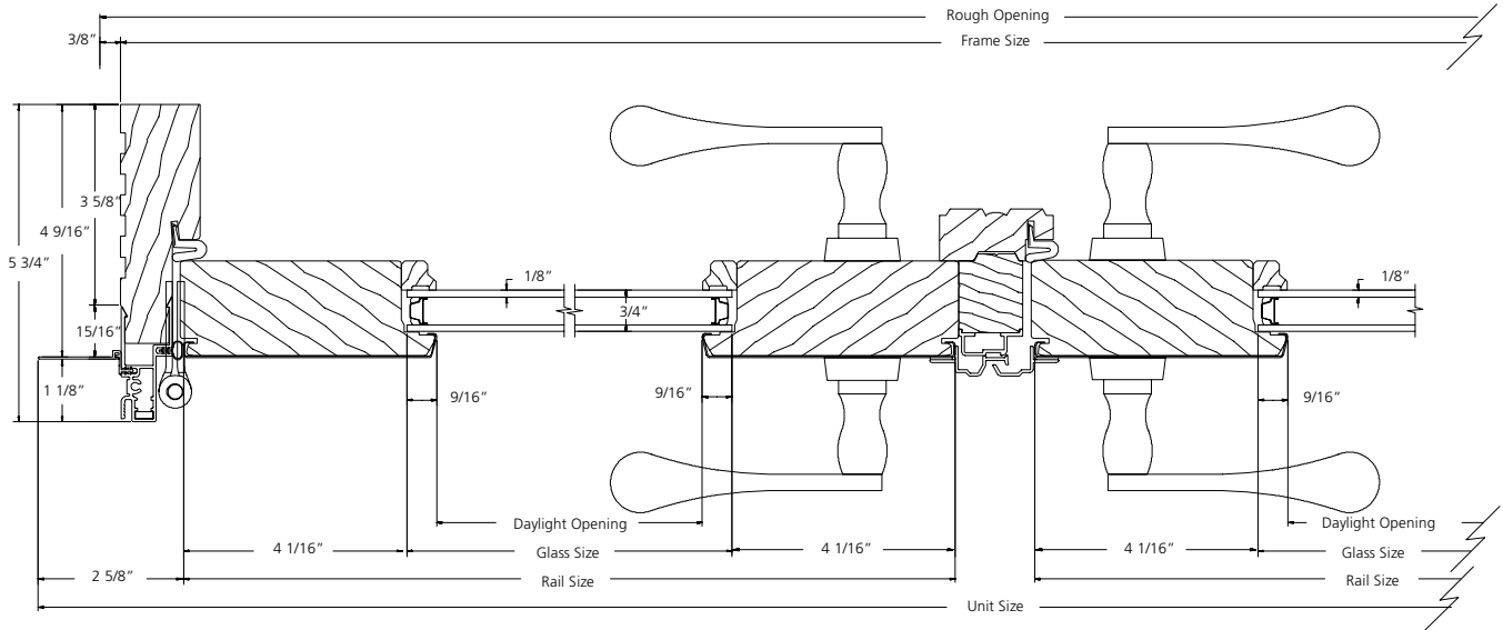
HORIZONTAL SECTION
