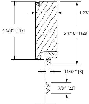
7/8" FULL SURROUND
