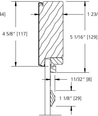
1 1/8" FULL SURROUND
