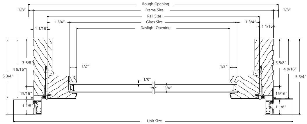
HORIZONTAL SECTION
