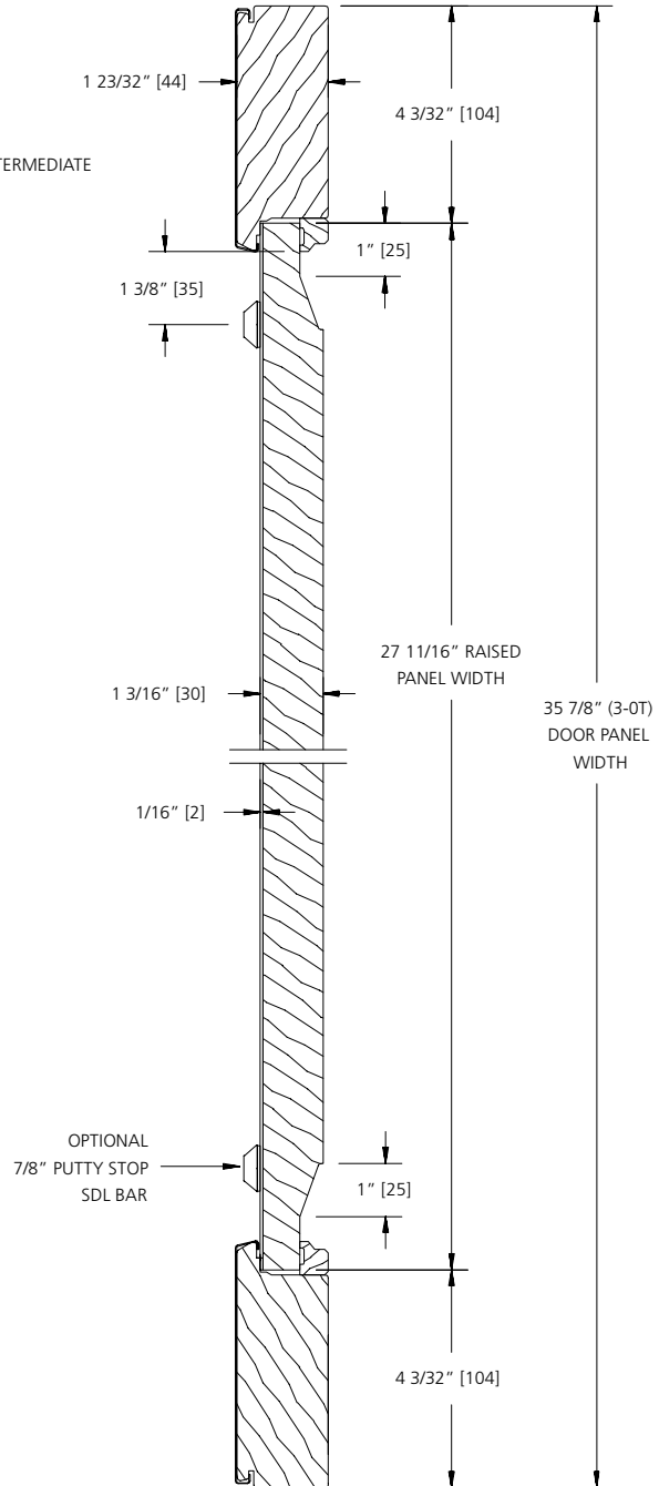
HORIZONTAL SECTION
