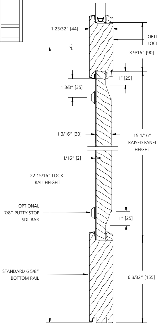
VERTICAL SECTION
