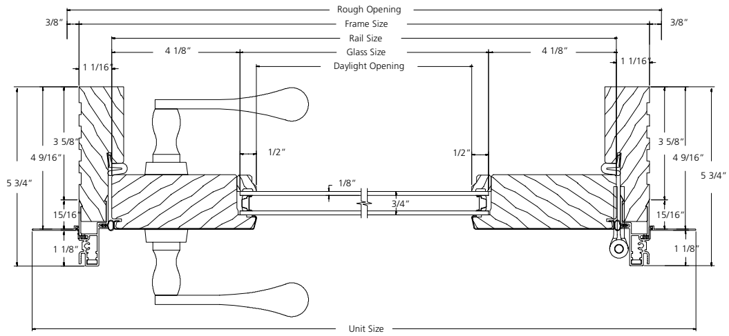
HORIZONTAL SECTION
