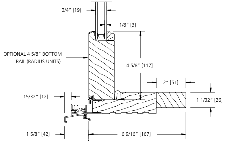
TRANSOM SILL NOSE (6 9/16" JAMB)
