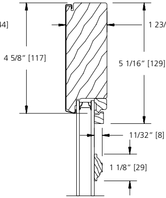
1 1/8" FULL SURROUND
