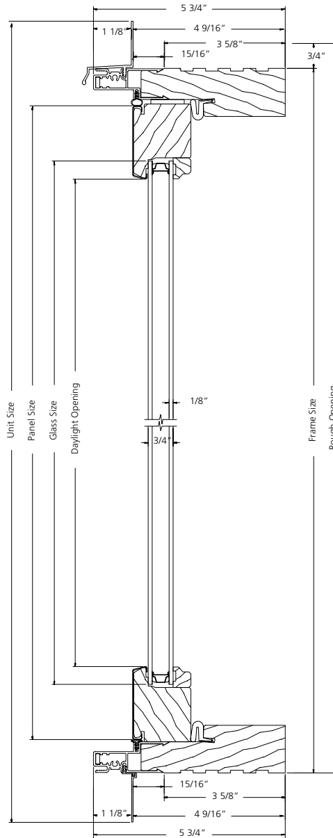
VERTICAL SECTION
