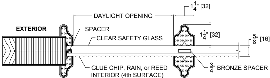
SIMULATED DIVIDED LITES - SDL (PATIO DOOR) SERIES GLUE CHIP, RAIN, or REED
