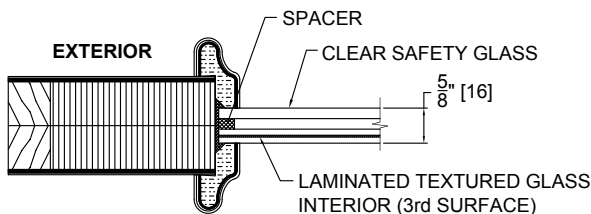
INSULATED GLASS LAMINATED TEXTURED (Including: Antique, Baroque, Cathedral Rose, Flash White, Gotta, Granite, Krinkle, Opal, Ripple, Seedy, Water, Weave, Wispy White)
