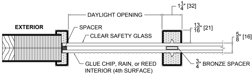
SIMULATED DIVIDED LITES - CRAFTSMAN SERIES GLUE CHIP, RAIN, or REED
