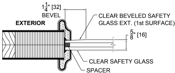
INSULATED GLASS BEVELED
