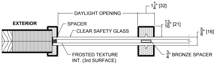
SIMULATED DIVIDED LITES - CRAFTSMAN SERIES FROSTED
