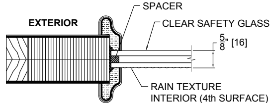
INSULATED GLASS RAIN
