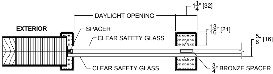
SIMULATED DIVIDED LITES - CRAFTSMAN SERIES CLEAR SAFETY
