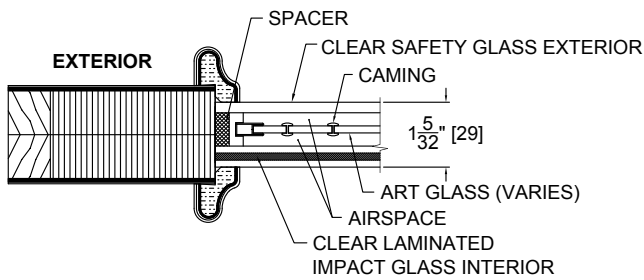
TRIPLE GLAZED IMPACT ART GLASS
