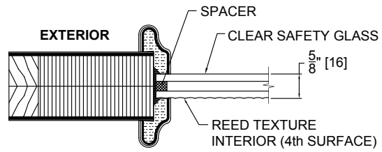
INSULATED GLASS REED
