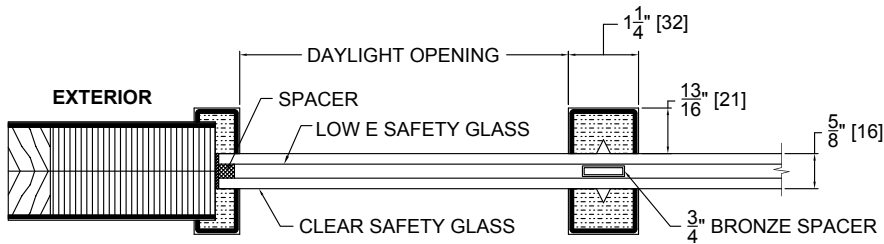
SIMULATED DIVIDED LITES - CRAFTSMAN SERIES LOW E
